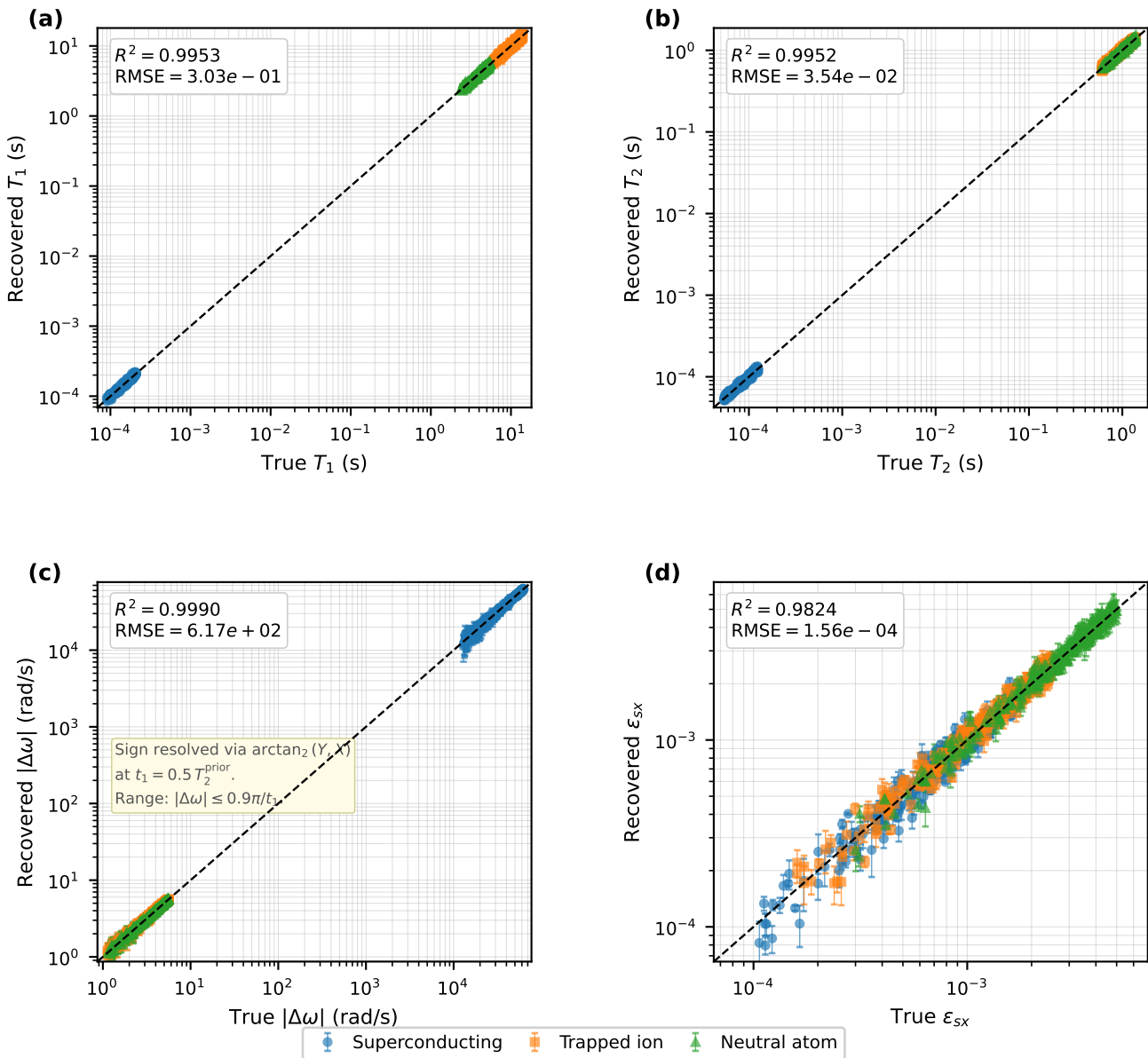
Fig. 2 — Parameter Recovery Accuracy (Digital Twin, N = 300/\text{arch} , seed=42, 9600 shots/qubit)
