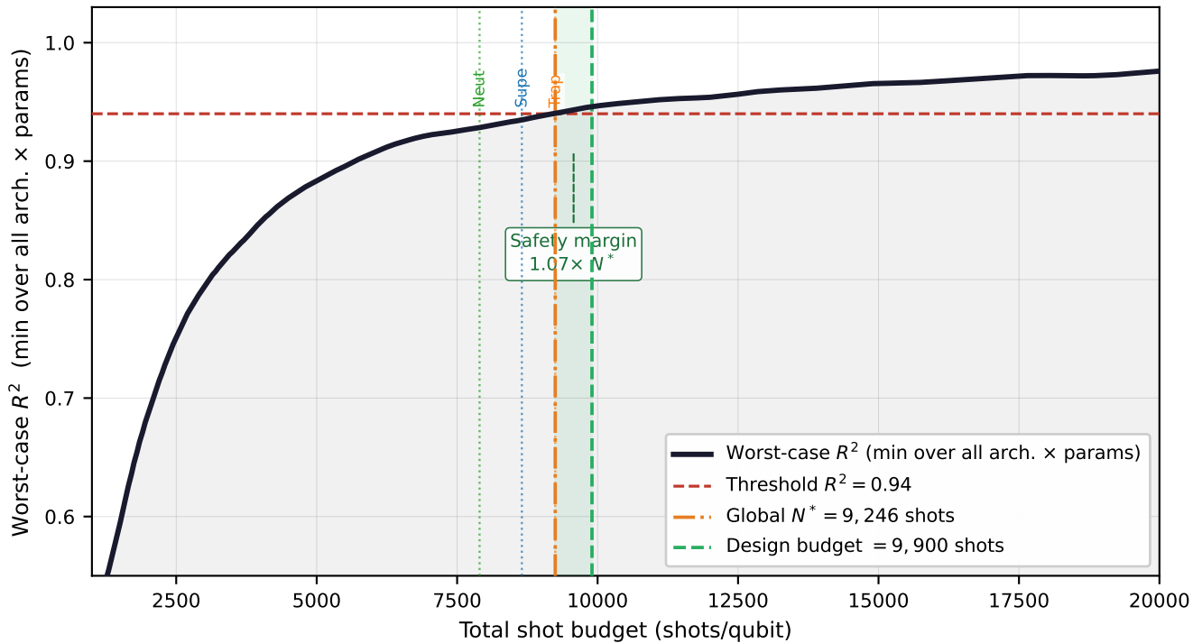
Fig. 4 — Shot-Budget Efficiency ( N^* = 9,246 shots, design = 9,900 shots, safety = 1.07 \times N^* )
