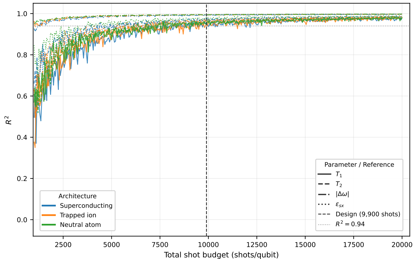
Fig. 4 — Shot-Budget Efficiency (3 architectures \times 4 parameters, N = 100/\text{budget} , seed=42)
