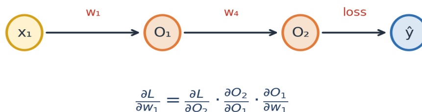
Figure 3.4 — The chain rule multiplies the step-by-step effects to find how a deep weight influences the loss.
