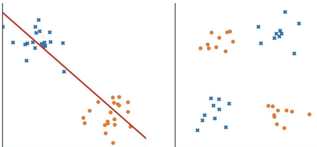
Figure 2.3 — Left: one straight line works. Right: no straight line works — we need multiple layers.
