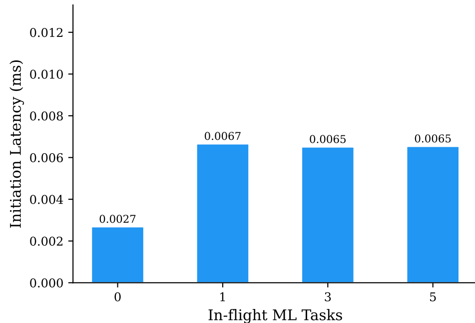
Broker Decision Overhead
