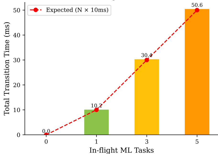
End-to-End Reallocation Latency (includes graceful drain)
