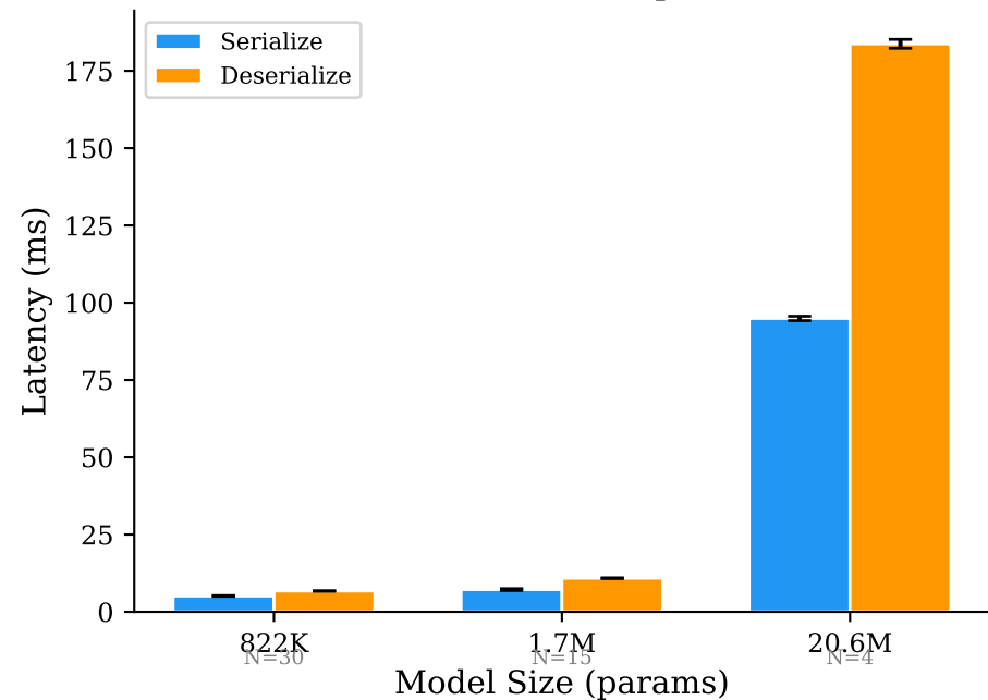
Redis Serialization Latency (real CVAE checkpoints)
