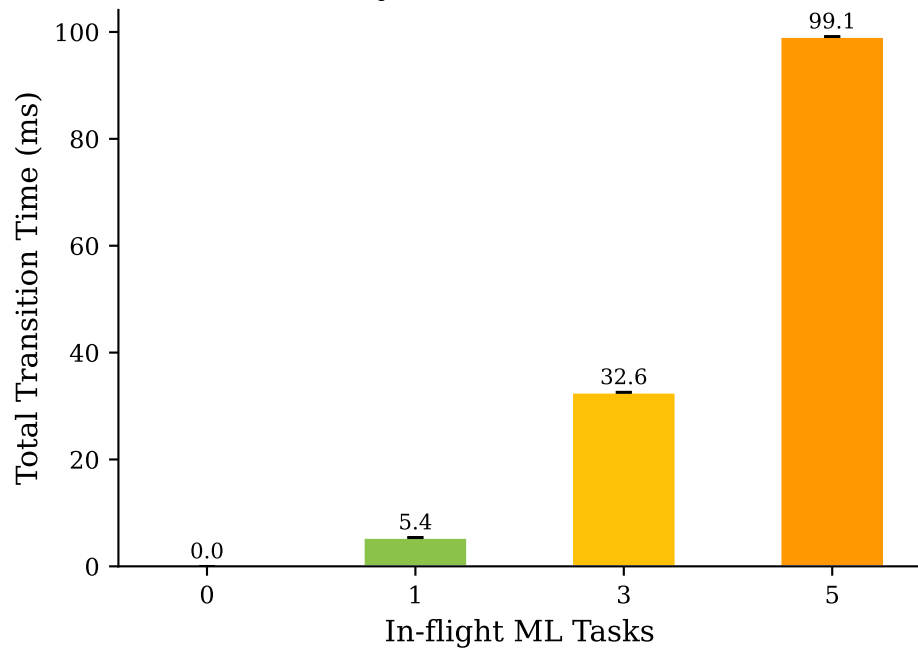
End-to-End Reallocation Latency (drain delays from real train durations)
