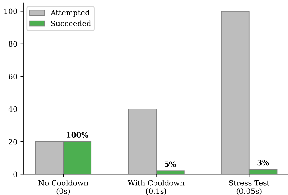
Cooldown Throttling Effect
