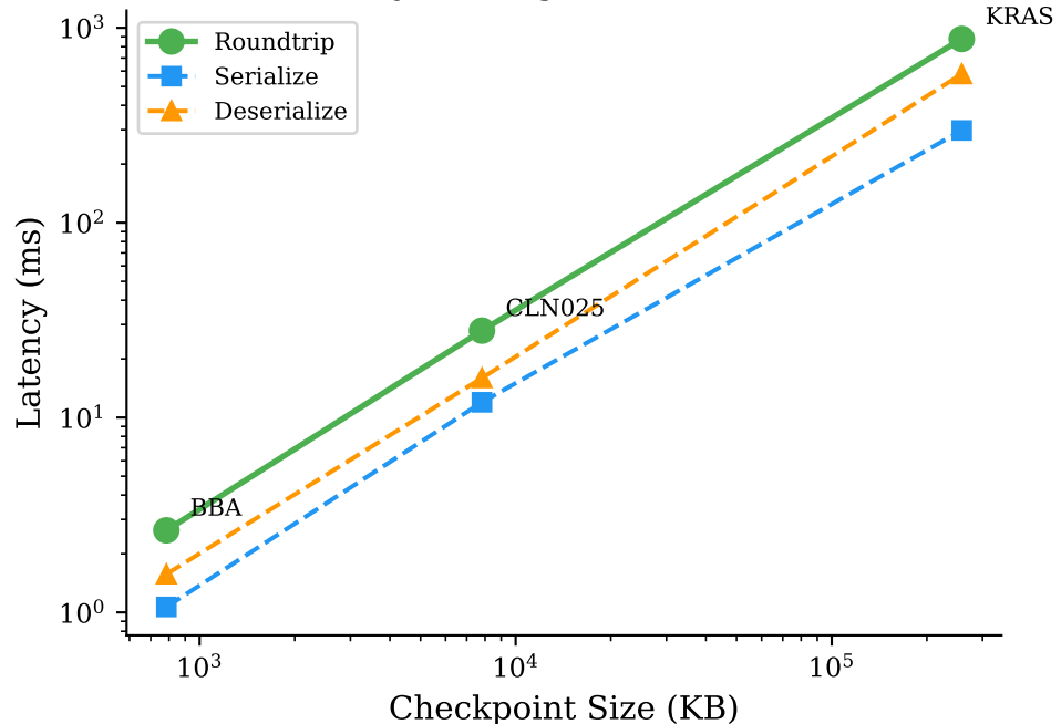
Latency Scaling with Model Size
