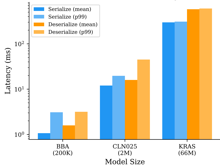
Redis Serialization Latency
