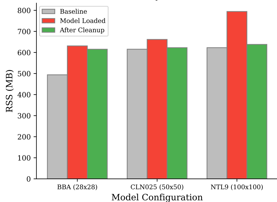
Worker Memory at Each Phase
