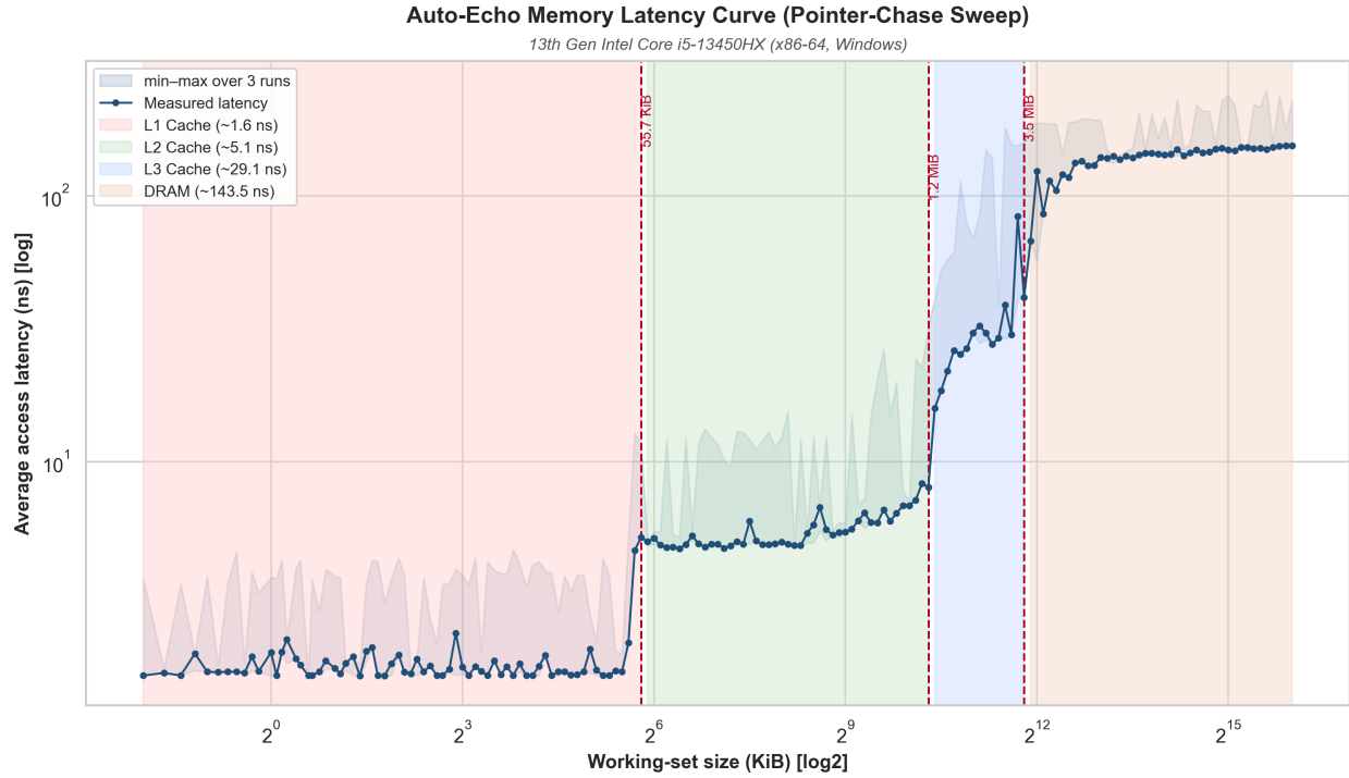
Fig. 7. Pointer-chase latency vs. working-set size on the Intel i5-13450HX performance core (minimum over three sweeps; the light band is the min-max spread). L1 (~48 KiB) and L2 (~1.25 MiB) are cleanly and stably resolved; beyond ~1.3 MiB TLB/page-walk latency dominates and the curve saturates at ~143 ns before the 20 MiB L3 can appear, so the third shaded band is a TLB-transition region rather than the L3 cache.
