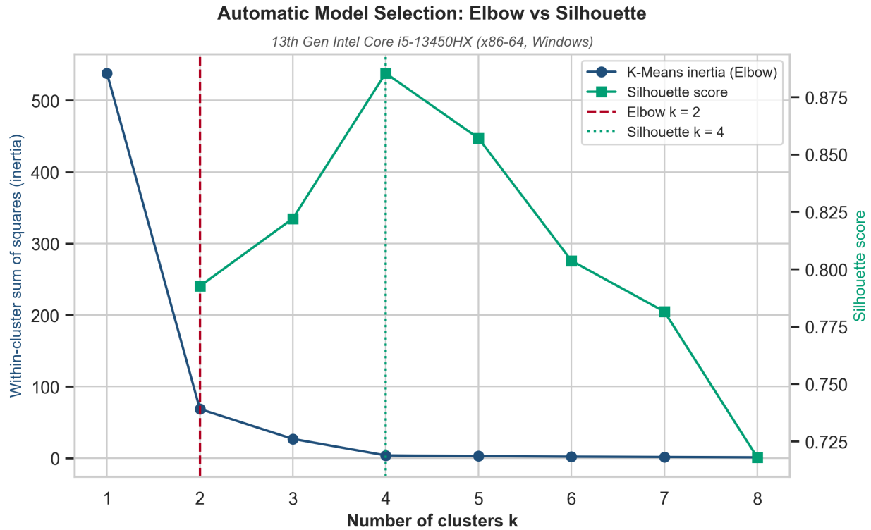
Fig. 8. Automatic model selection on the Intel i5-13450HX: the K-Means inertia elbow selects k = 2 while the Silhouette score peaks at k = 4 — the two criteria disagree , the model-selection signature of the unstable x86 level
