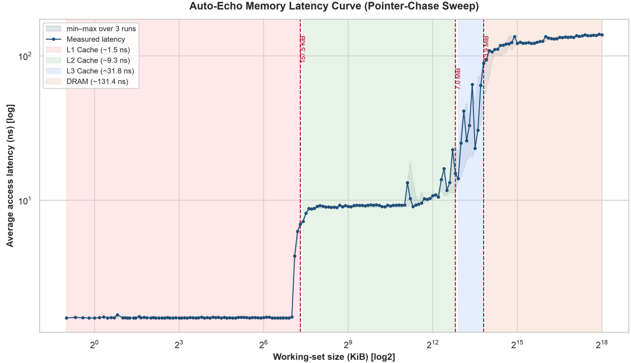
Fig. 1. Pointer-chase latency vs. working-set size (log-log). Shaded bands are the detected levels;
