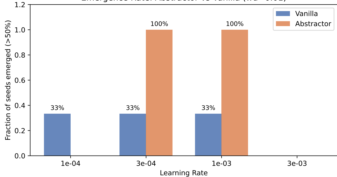
Emergence Rate: Abstractor vs Vanilla (wd=0.01)
