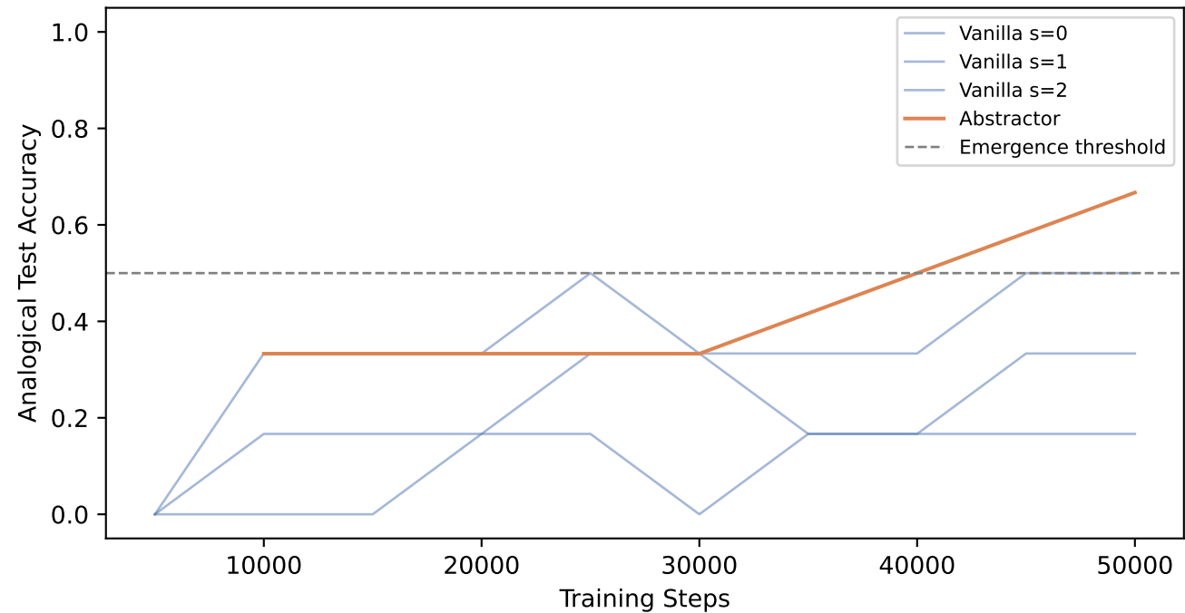
Grokking: Vanilla vs Abstractor (lr=1e-03, wd=0.01)
