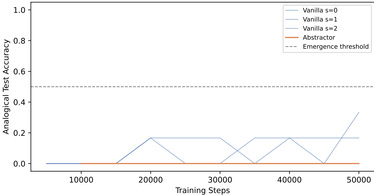
Grokking: Vanilla vs Abstractor (lr=3e-03, wd=0.01)
