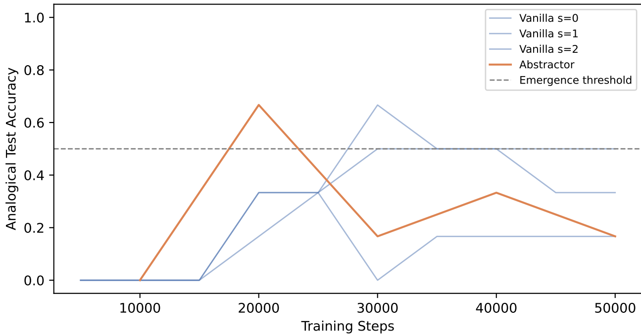
Grokking: Vanilla vs Abstractor (lr=3e-04, wd=0.01)
