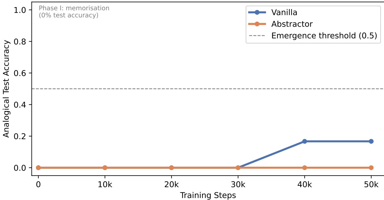
Grokking Dynamics: Vanilla vs Abstractor ( \text{lr}=3\text{e-}03 , \text{wd}=0.01 , \text{seed}=0 )
