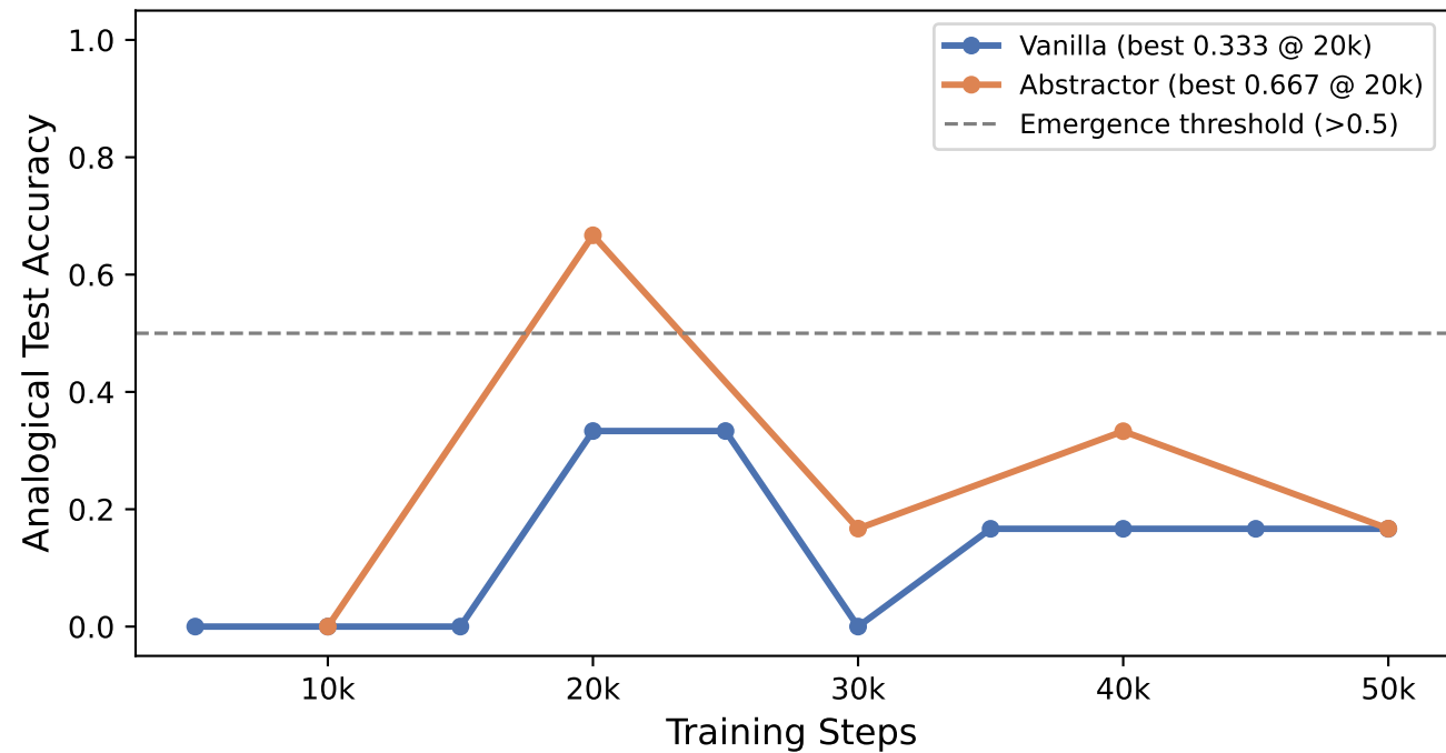
Grokking: Vanilla vs Abstractor (LR=3e-4, seed=0, wd=0.01)
