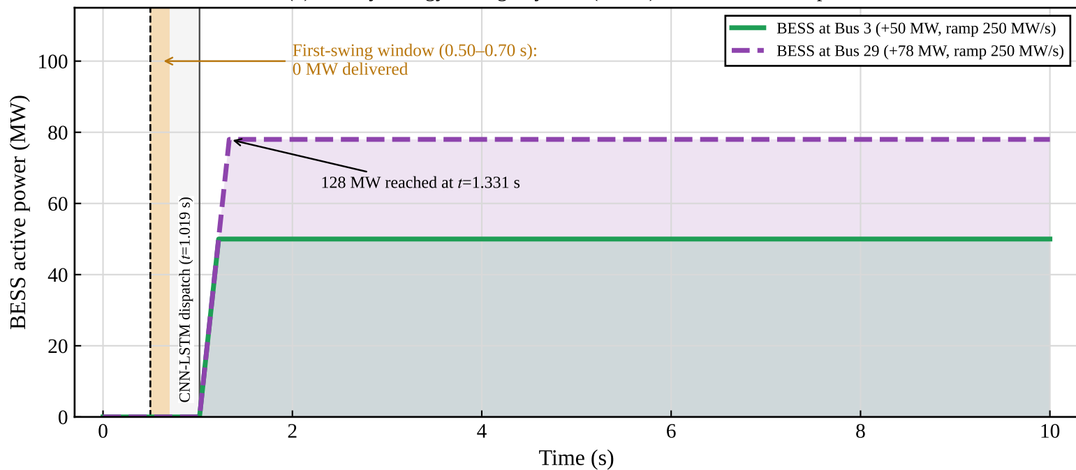
(b) Battery Energy Storage System (BESS) Active-Power Response
