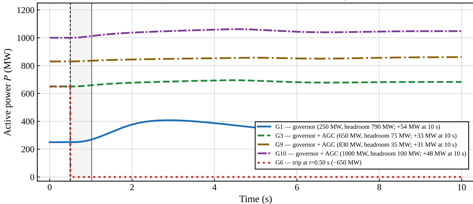
(a) Synchronous Generator Active Power (Table 4 set-points)
