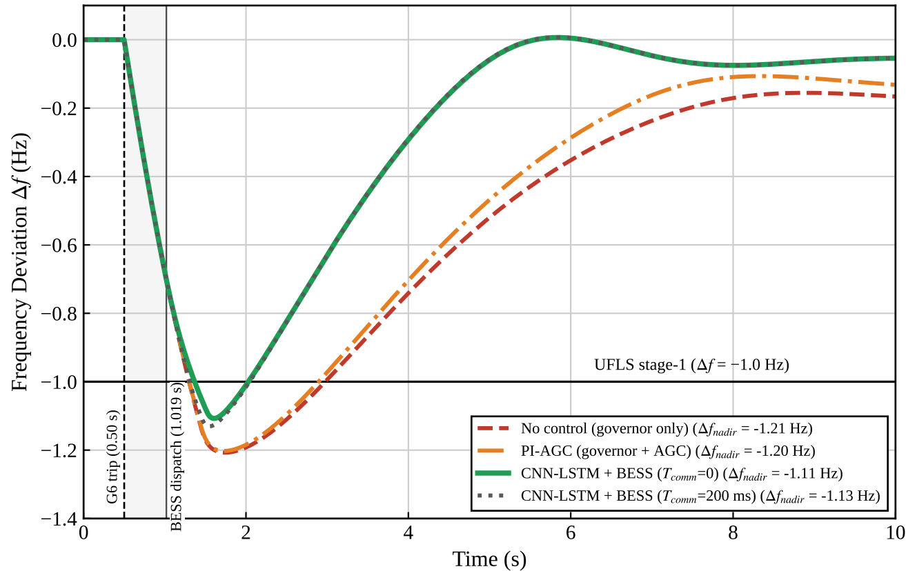
(a) IEEE 39-Bus: Control Comparison
