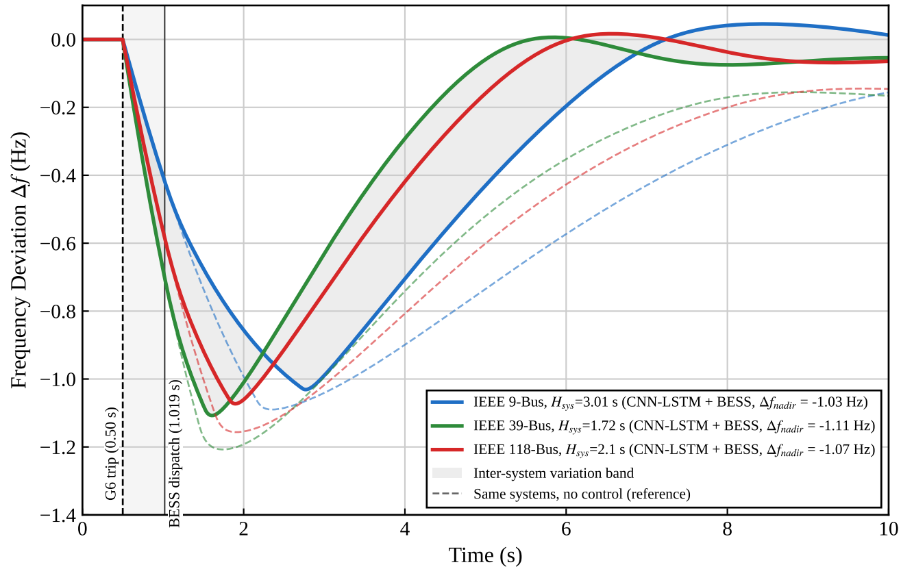
(b) CNN-LSTM + BESS Across Test Systems (10.3% generation loss)
