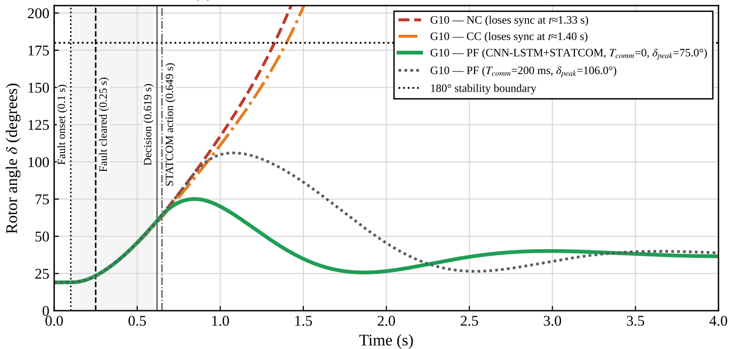
(b) G10 — With and Without CNN-LSTM Corrective Control
