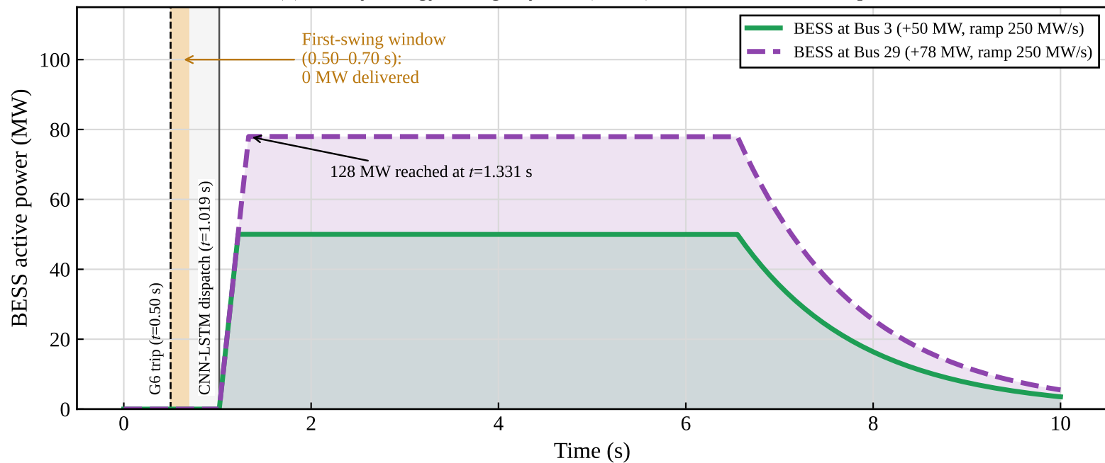
(b) Battery Energy Storage System (BESS) Fast Active-Power Response
