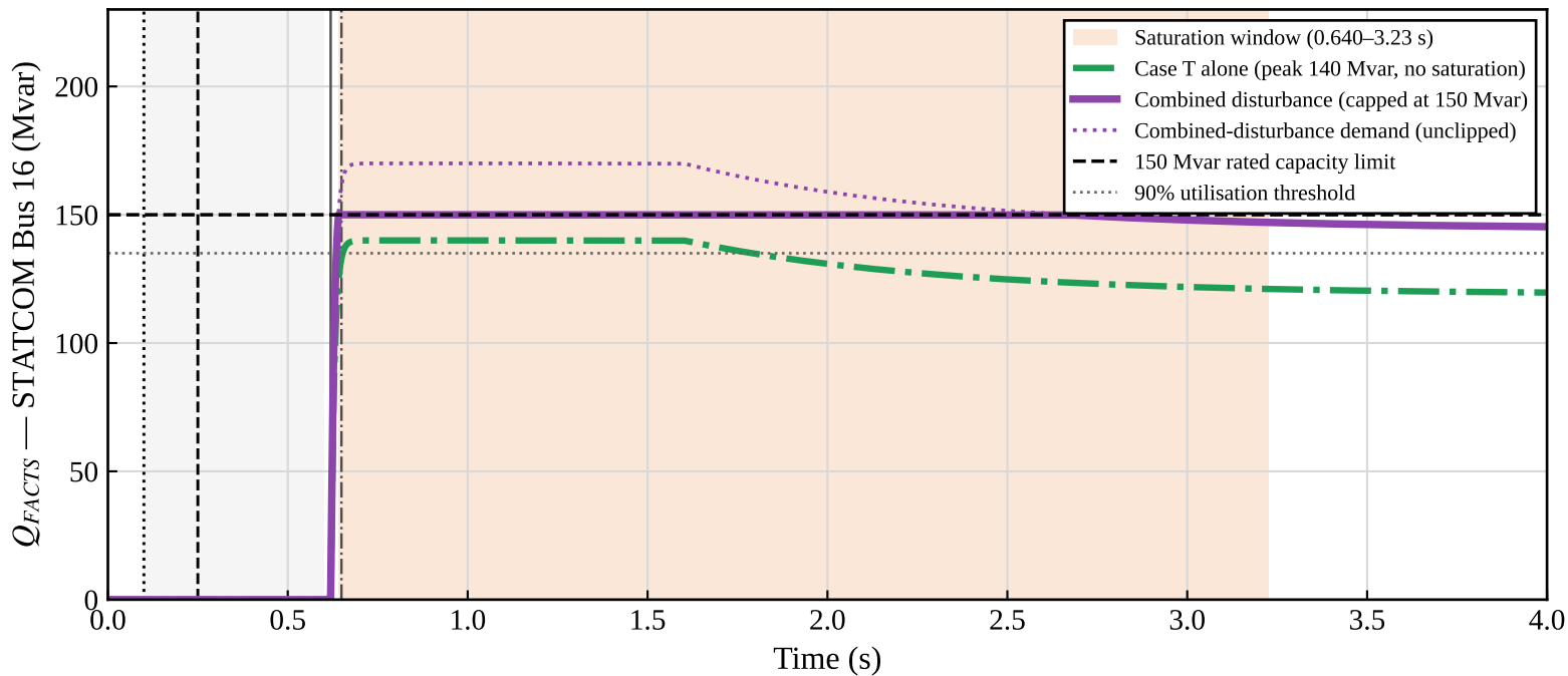
(b) STATCOM Reactive-Power Output — Saturation Clamping Visible
