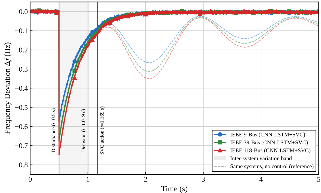
(b) CNN-LSTM+SVC Across Test Systems
