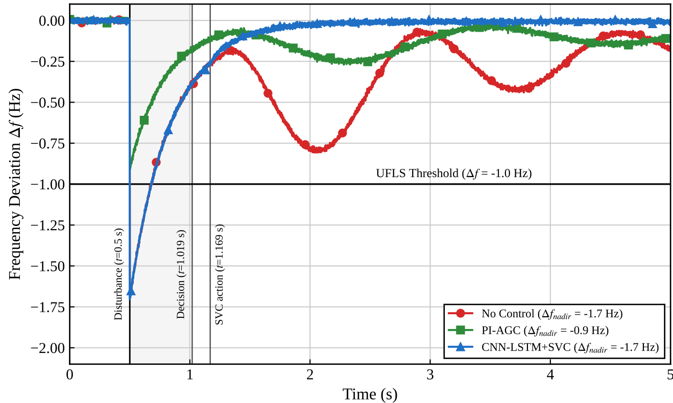
(a) IEEE 39-Bus: Control Comparison
