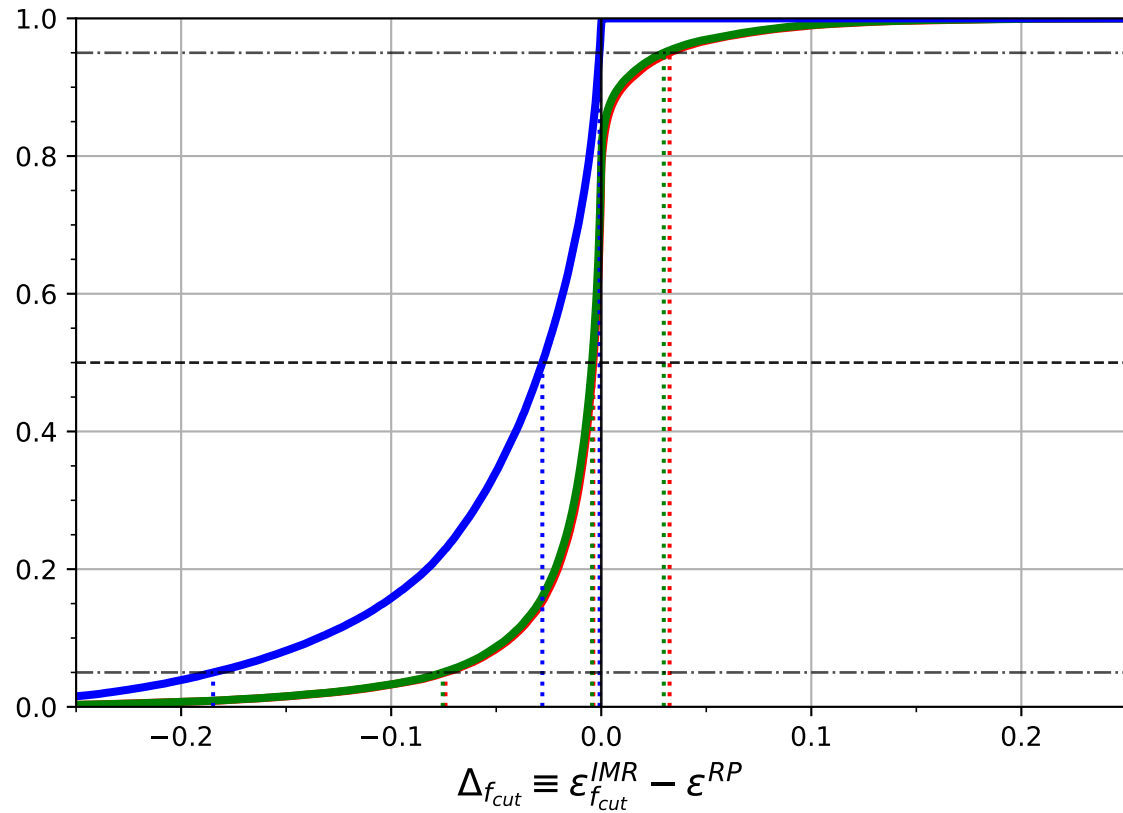
Cumulative Distribution
