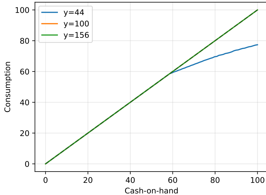
Consumption Policy
