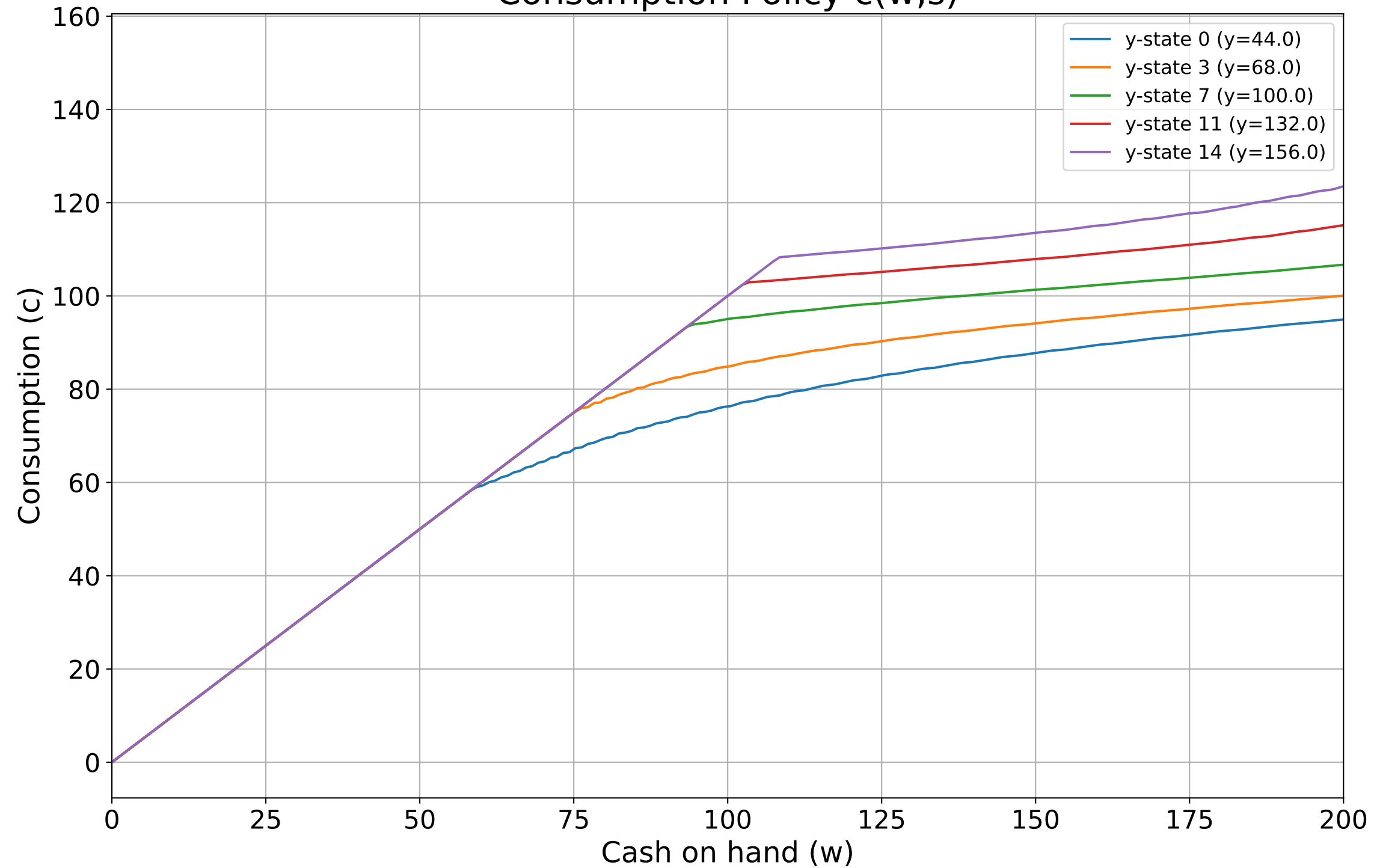
Consumption Policy c(w,s)
