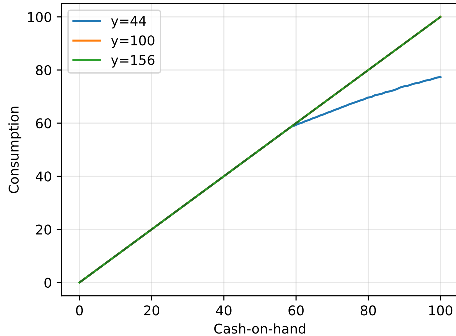
Consumption Policy
