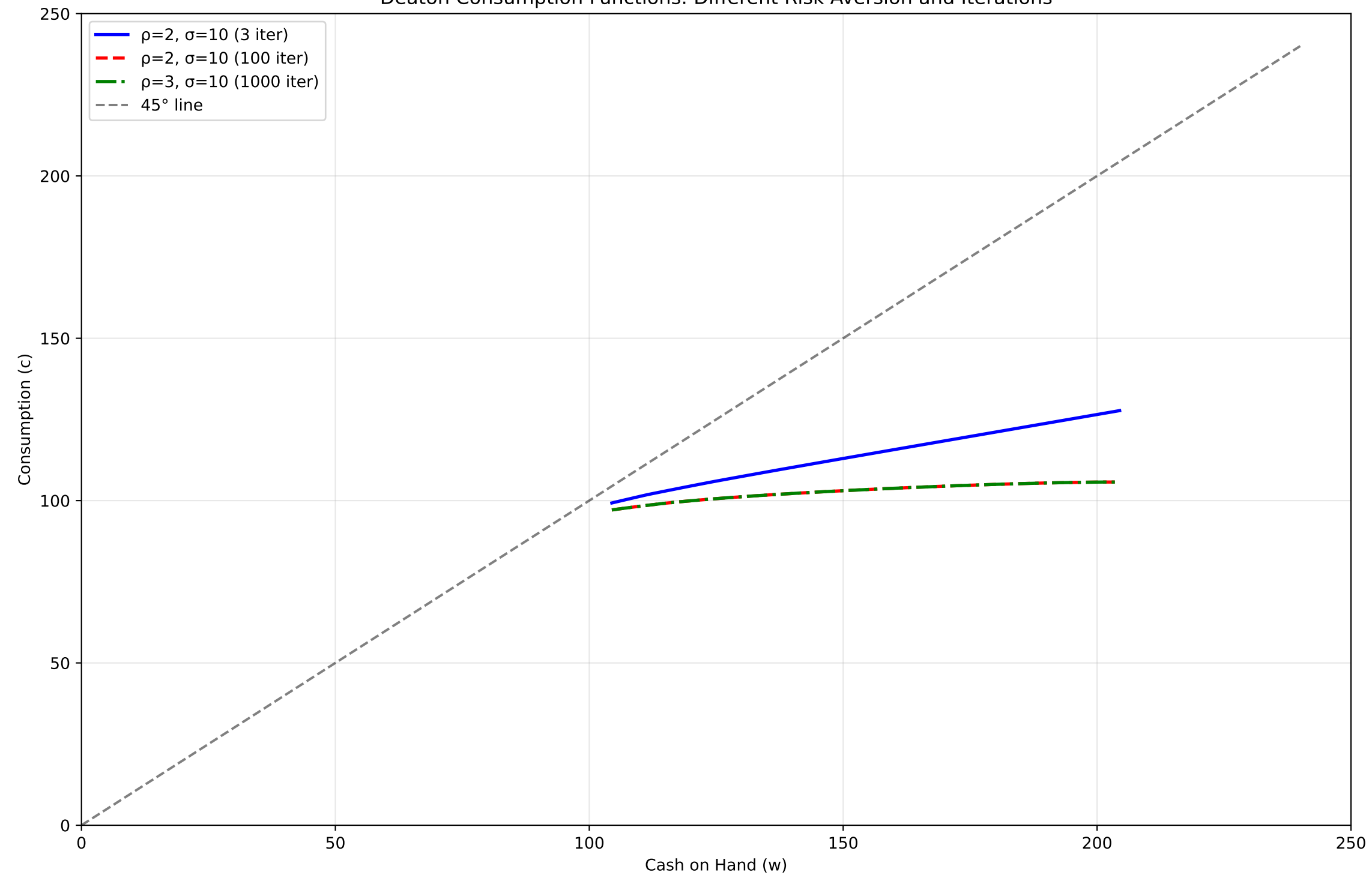
Deaton Consumption Functions: Different Risk Aversion and Iterations
