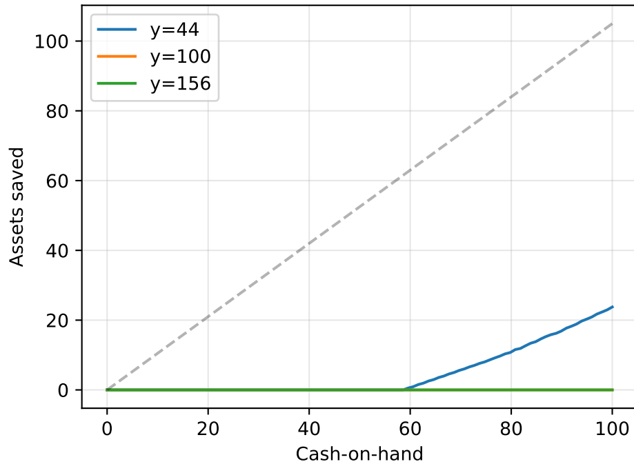
Savings Policy
