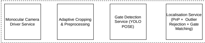
T1 : The Vision Pipeline (Runs at 30–90 Hz on Jetson GPU/CPU)
