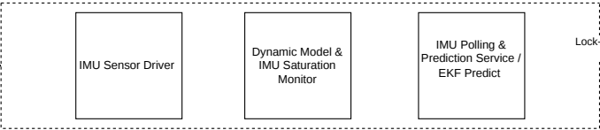
T2 : High-Frequency IMU & Prediction (Runs at 1,000–2,000 Hz on Jetson CPU)
