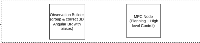
T4 : The Planning & Control Loop (Runs at 50–100 Hz on Jetson CPU)
