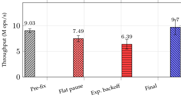
Fig. 4. numaring_sustained_load throughput at 32 threads, same host (Table 4): mean of three 15-second runs, error bars span the observed range. Both backoff variants (red) sit below the pre-fix baseline (gray); the work-stealing fix with no backoff (blue) is the only variant that improves on it.
