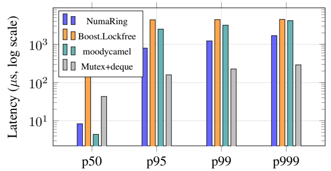
Figure 2: p50/p95/p99/p99.9 latency at 32 threads, same host, current build. See Table 3 for the exact values plotted.
