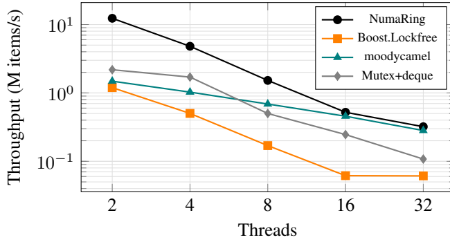
Figure 1: Throughput vs. thread count, same host, current build. All four implementations run the identical timestamp-payload workload through the identical harness.
