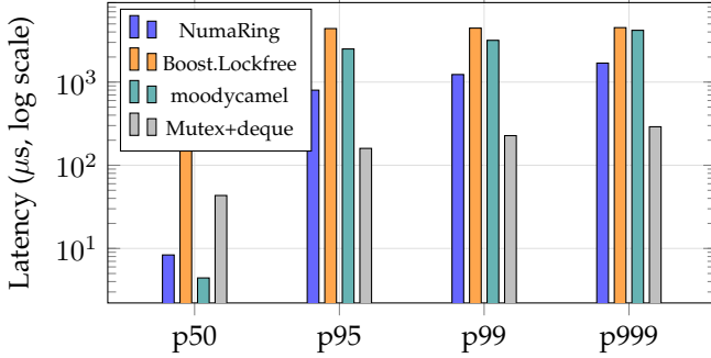
Fig. 2. p50/p95/p99/p99.9 latency at 32 threads, same host, current build. See Table 3 for the exact values plotted.
