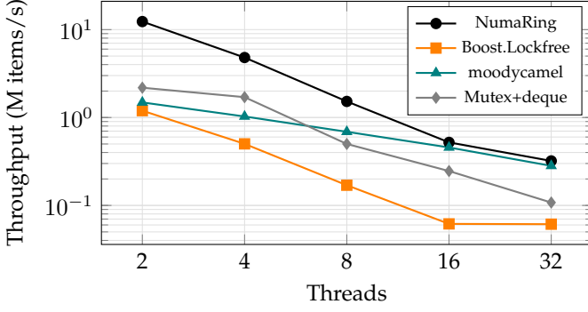
Fig. 1. Throughput vs. thread count, same host, current build. All four implementations run the identical timestamp-payload workload through the identical harness.
