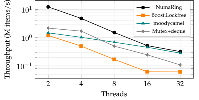
Fig. 2. Throughput vs. thread count, same host, current build. All four implementations run the identical timestamp-payload workload through the identical harness.
