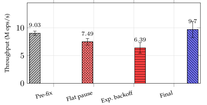
Fig. 4. numaring_sustained_load throughput at 32 threads, same host (Table 4): mean of three 15-second runs, error bars span the observed range. Both backoff variants (red) sit below the pre-fix baseline (gray); the work-stealing fix with no backoff (blue) is the only variant that improves on it.
