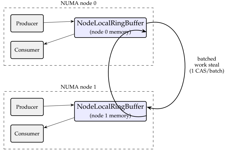
Fig. 1. NumaRing’s two-node architecture. Producers and consumers route to their own node’s ring buffer via current_node() (Section 3.2); the fast path never crosses the dashed boundary. Batched work stealing (Section 3.3) only runs when a node’s ring is locally full or empty.
