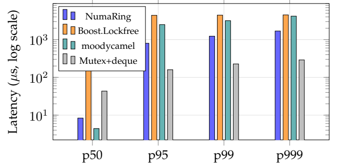
Fig. 3. p50/p95/p99/p99.9 latency at 32 threads, same host, current build. See Table 3 for the exact values plotted.
