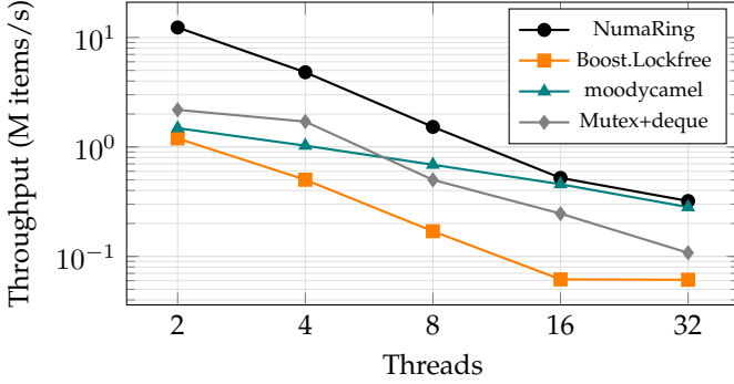
Fig. 2. Throughput vs. thread count, same host, current build. All four implementations run the identical timestamp-payload workload through the identical harness.
