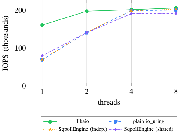
Fig. 2. IOPS versus thread count at queue depth 32, 16 vCPUs (Table II). libaio’s lead is widest at a single thread; every backend converges near the device ceiling by 4 threads.
