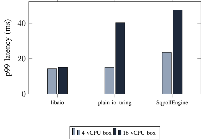
Fig. 3. p99 latency at 4 threads, queue depth 128, 4-vCPU versus 16-vCPU box (Table III). libaio’s tail barely moves; both io_uring-based backends get worse on the wider machine.
