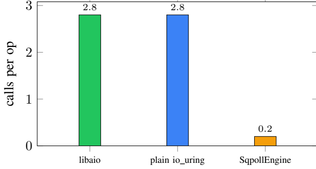
Fig. 1. Round trips per completed operation at 4 threads, queue depth 128. Bars for libaio and plain io_uring plot the midpoint of their reported 1.3–4.3 range; Table I has the exact figures.
