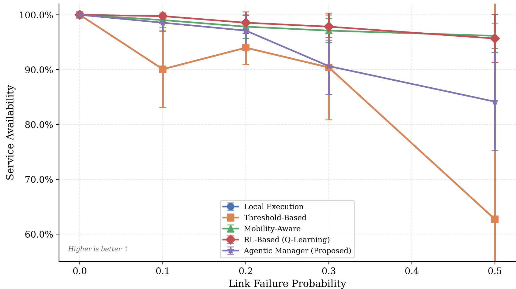
Service Availability Under Varying Connectivity Reliability
