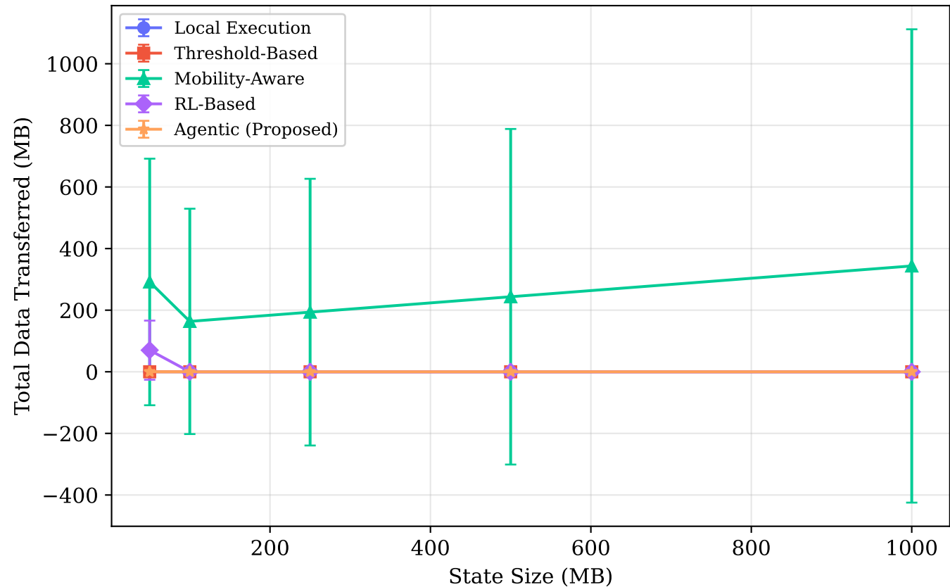
Fig 3: Migration Overhead vs State Size
