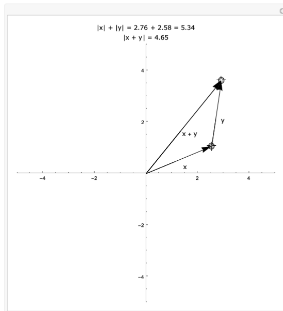
Figure 1.2: visualization of the triangle inequality; |x + y| \leq |x| + |y| for all x, y \in \mathbb{R} .
