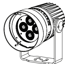
Exterior Wash 110 with snoot
