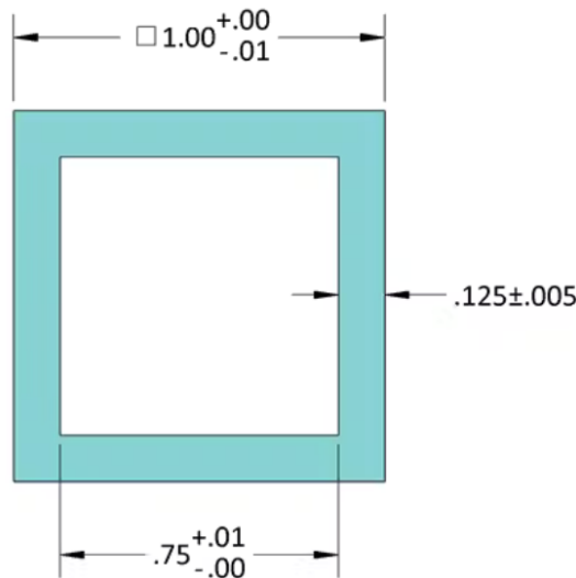
Figure 9.1: Basic Dimensions with size tolerances of a box shape. Lengths, denoted by a pair of arrows, are listed alongside a numerical measurement, typically associated with a unit convention such as imperial or metric. The tolerance, denoted by the plus/minus sign, writes the maximum and minimum lengths of the part.
