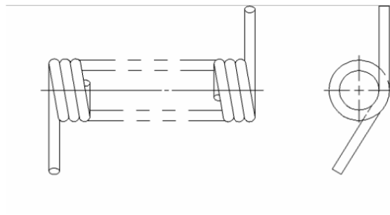
Figure 9.4: Coiled spring with repeated details.
