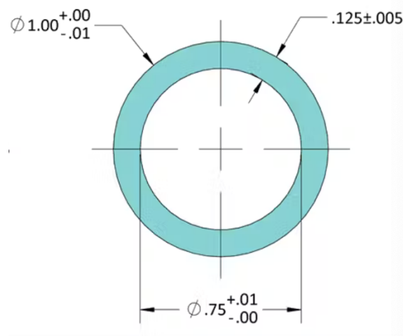
Figure 9.2: Basic Dimensions with size tolerances of a circular shape. Lengths, denoted by a pair of arrows, are listed alongside a numerical measurement, typically associated with a unit convention such as imperial or metric. The tolerance, denoted by the plus/minus sign, writes the maximum and minimum lengths of the part. The diameter of the circle is noted by the symbol \phi , which explicitly states the diameter of the shape. Here, pictured is the nominal diameter, or outer-diameter abbreviated OD. The ordinal diameter, or inner-diameter abbreviated ID.
