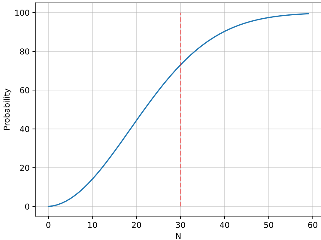
Probability at least 2 Birthday Overlaps
