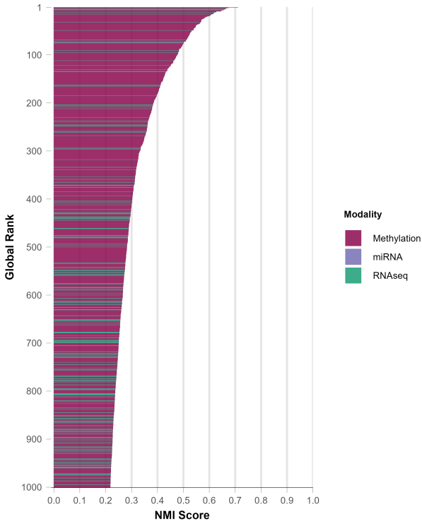
Top 1000 Features Ranked by NMI with Subtypes
