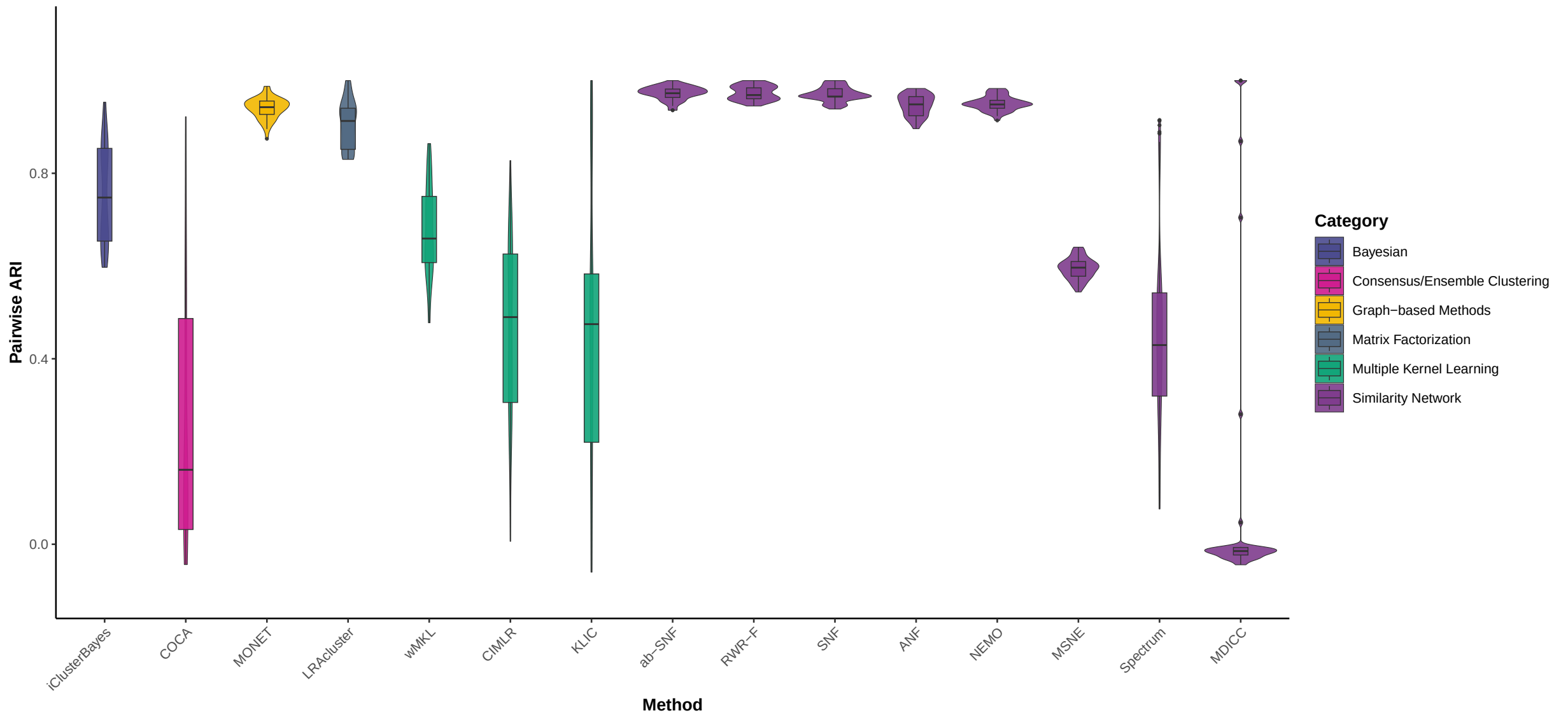
Replicate stability at 90% sample perturbation
