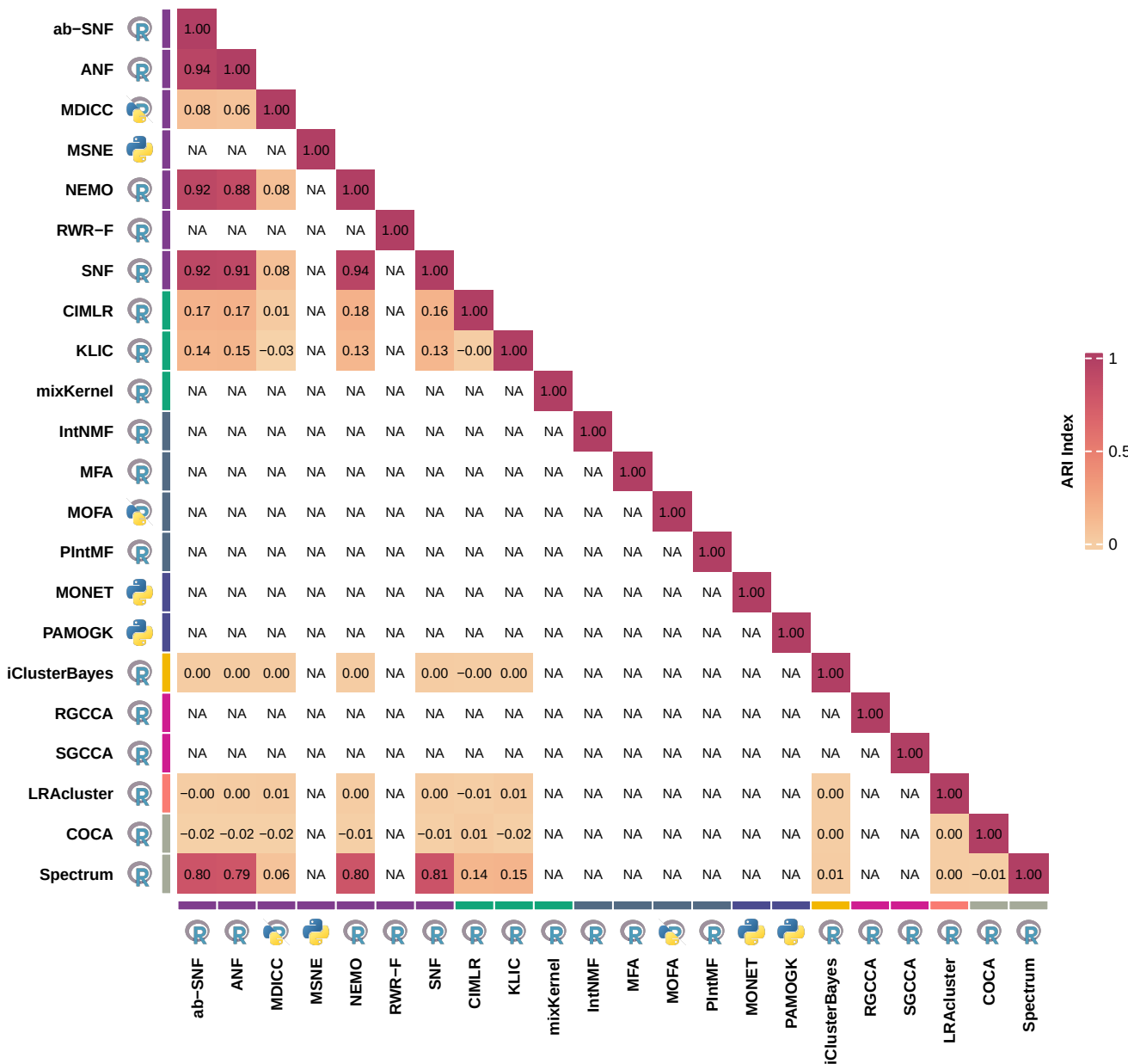
Adjusted Rand Index (ARI) between clusterings
