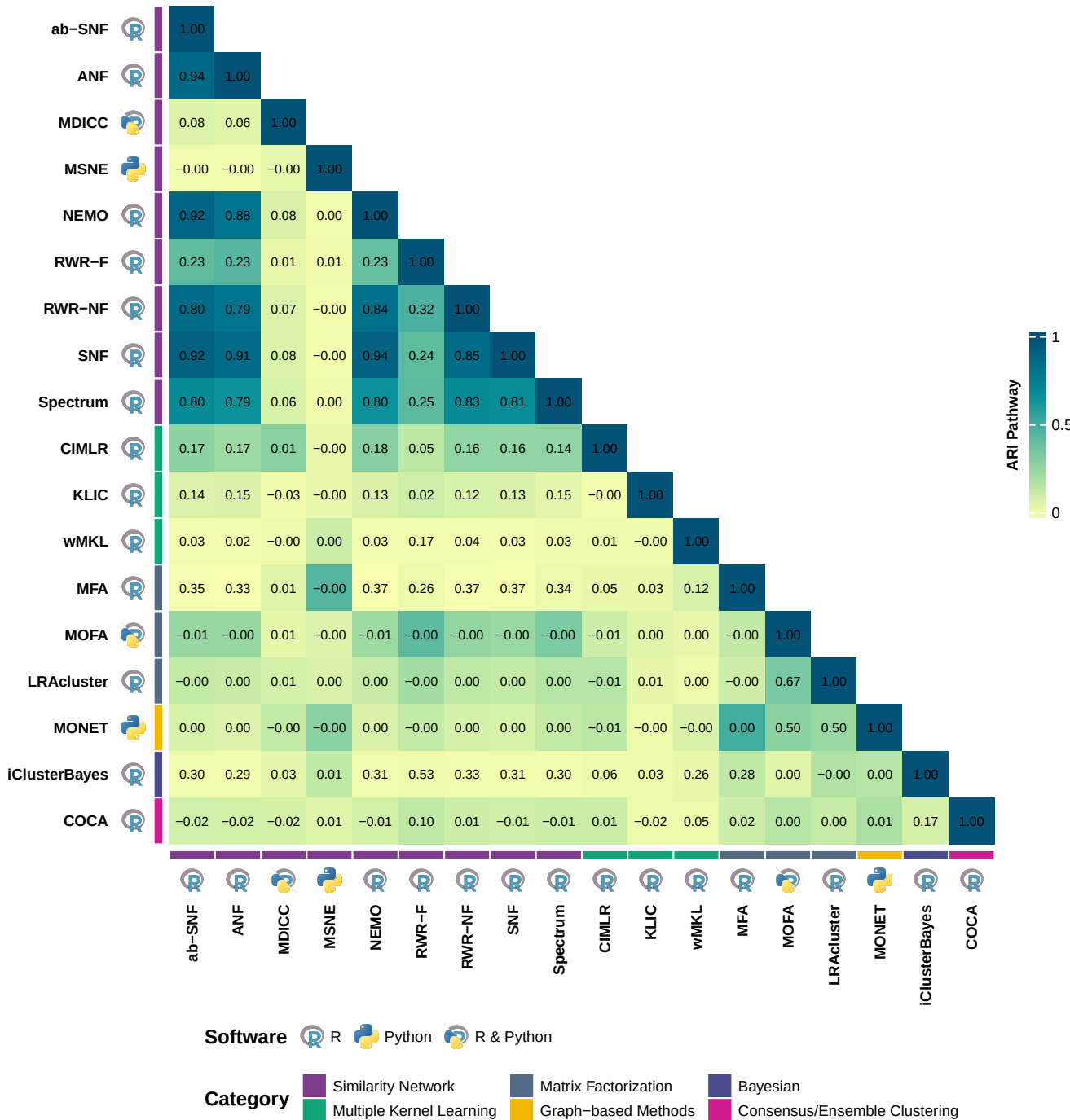
Adjusted Rand Index (ARI) for Aggregated Pathways
