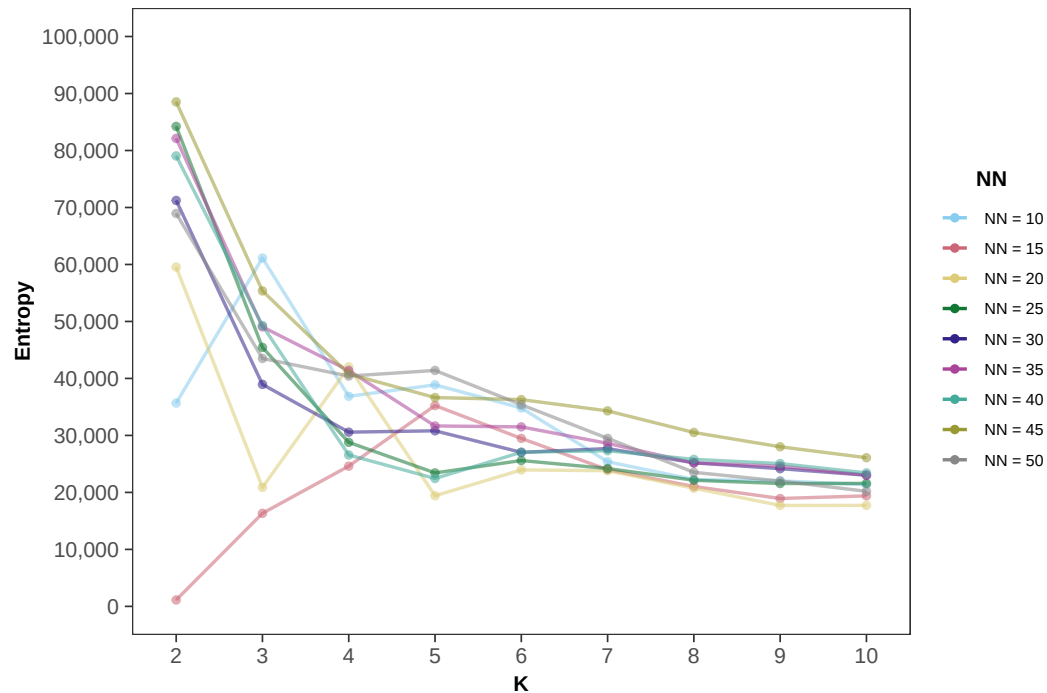
Entropy in Real Data
