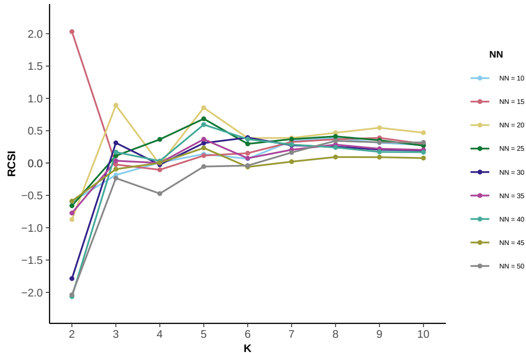
RCSI vs. number of clusters K for different NN values
