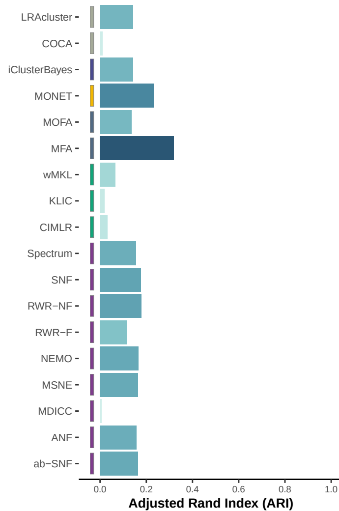
ARI bar chart: PARADIGM
