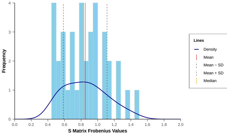
Histogram of Frobenius values between S matrices for different values of Nearest Neighbors
