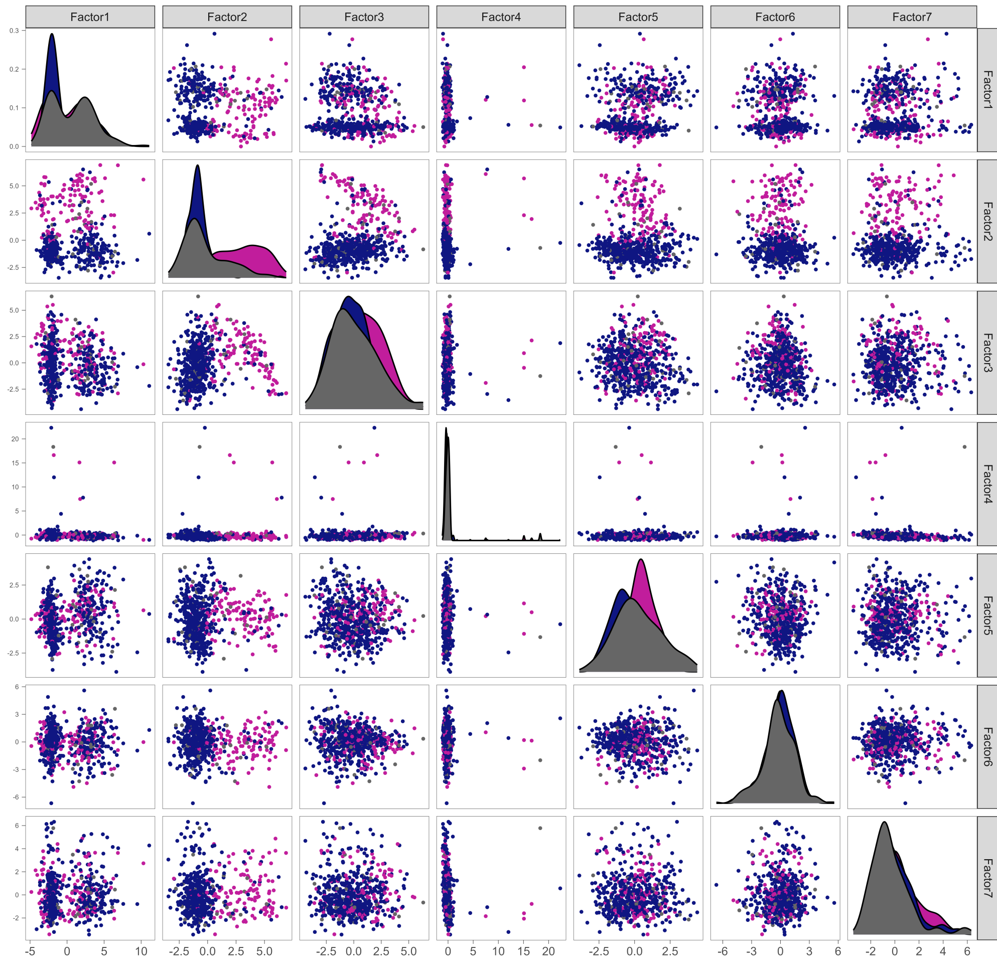
MOFA factors vs. ER status
