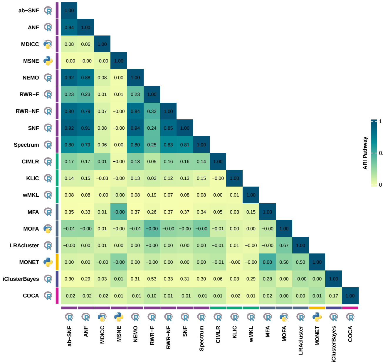
Adjusted Rand Index (ARI) for Aggregated Pathways
