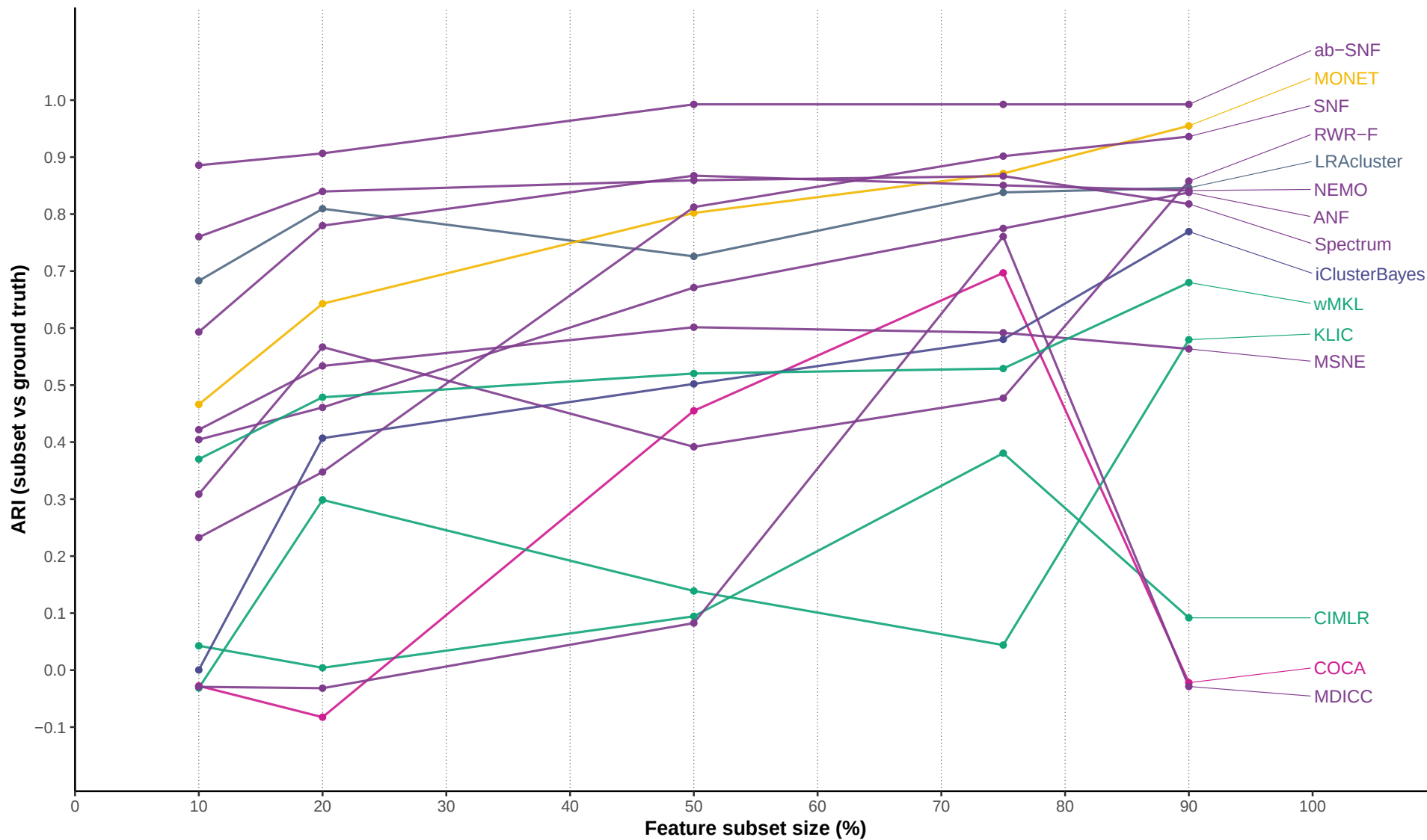
Agreement with ground-truth clustering under feature perturbations
